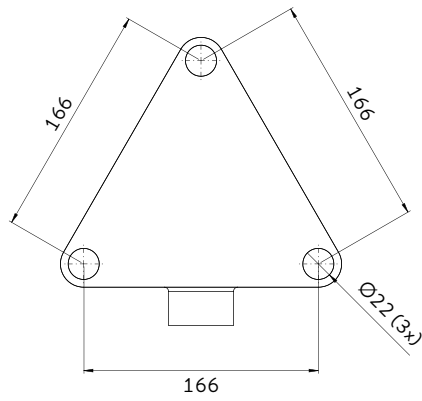
Markplate 5-12 m
